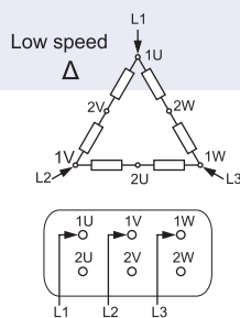
Highest output at both speeds, Dahlander connection
