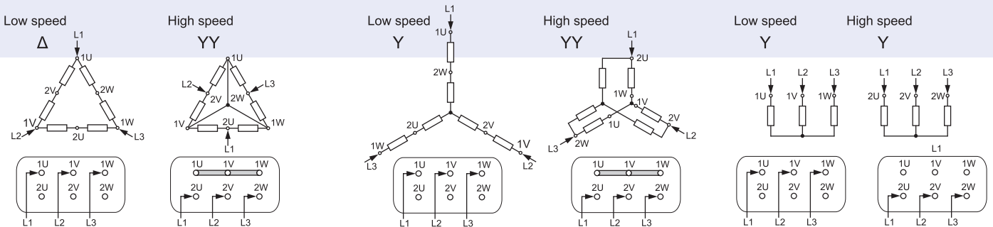
Highest output at both speeds, Dahlander connection
